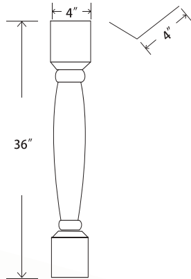
▲ Decorative Corbel — • DLS4*4*36"
