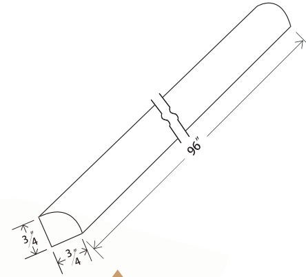
Shoe Molding
