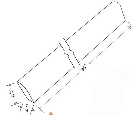
Scribe Molding
