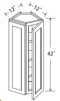
Wall End Corner Cabinet 42"H - 2 Doors, 3 shelves
