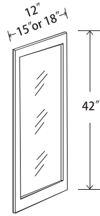
Wall Cabinet Single Glass Door, 42"H
