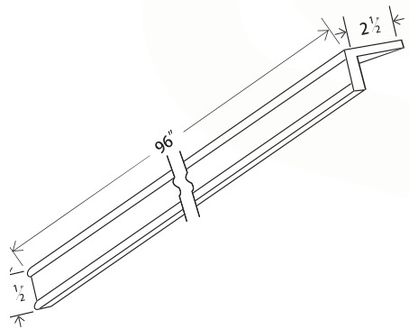
Light Rail Molding
