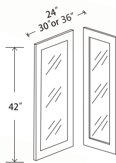
Wall Cabinet Double Glass Doors, 42"H
