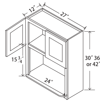
Microwave Wall Cabinet
