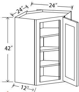
Diagonal Corner Wall Single Door 42"H
