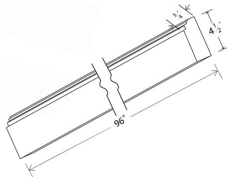
Base Molding
