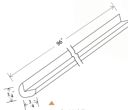
Angle Molding
