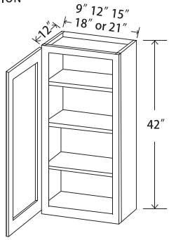
Wall Cabinet Single Door, 42"H
