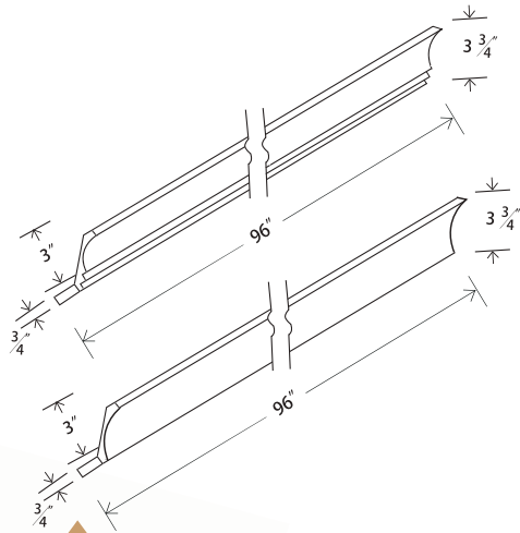
Crown Molding
